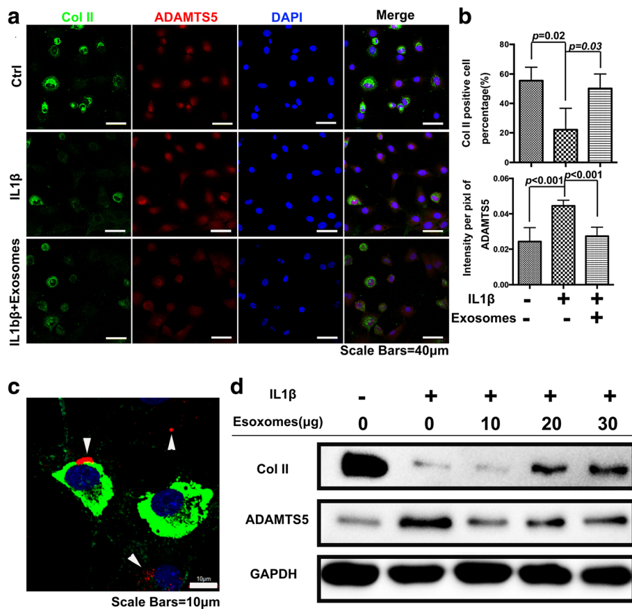
Fig. 5 Direct effects of exosomes on primary chondrocyte phenotype maintenance in the presence of IL-1 \beta . a Expression of Col II (green) and ADAMTS5 (red) by primary chondrocytes treated with exosomes. Scale bar, 40 \mu m. b Percentages of the Col II-positive cells with/without the addition of exosomes and immunofluorescence intensity of ADAMTS5 with/without the addition of exosomes. c Colocalization of exosomes (red), Col II (green) and chondrocytes (blue nuclei). Scale bars, 10 \mu m. d Expression of Col II and ADAMTS5 by the primary chondrocytes upon addition of different concentrations of exosomes. COL II collagen type II, IL-1 \beta , interleukin 1 beta
