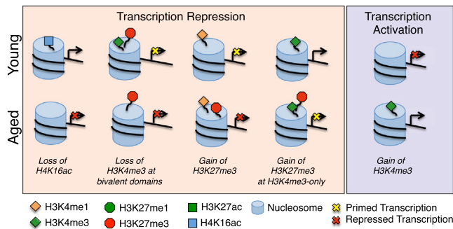
Figure 4. Histone Modifications in an Adult Stem Cell Compartment during Aging Cooperate to Influence Transcriptional Competence A schematic of histone modification dynamics in stem cells as a consequence of aging and their influence on gene expression. The complex histone code presents many combinations to repress, activate, or prime expression of transcripts.
