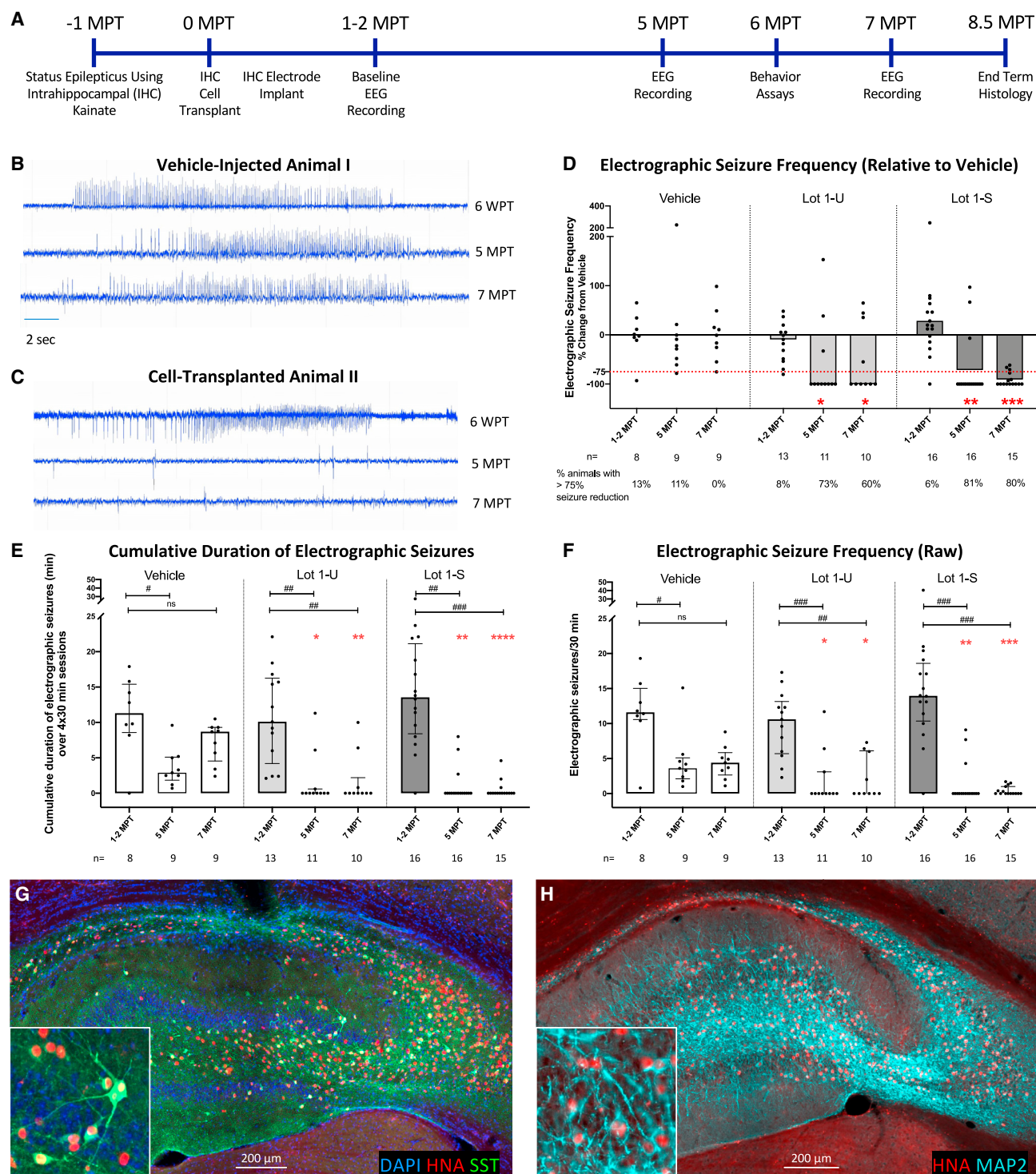
Figure 4. Seizure suppression after cell transplantation of lots 1-U and 1-S in the chronic MTLE mouse model
